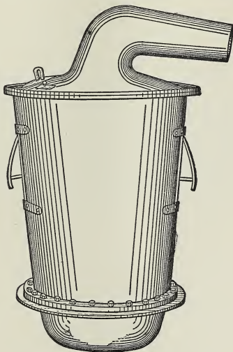
FIG. 14.—Heraeus' Varnish-kettle.
